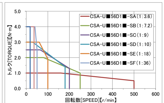
CSA-U ■ 56D1-S series [Geared type]
